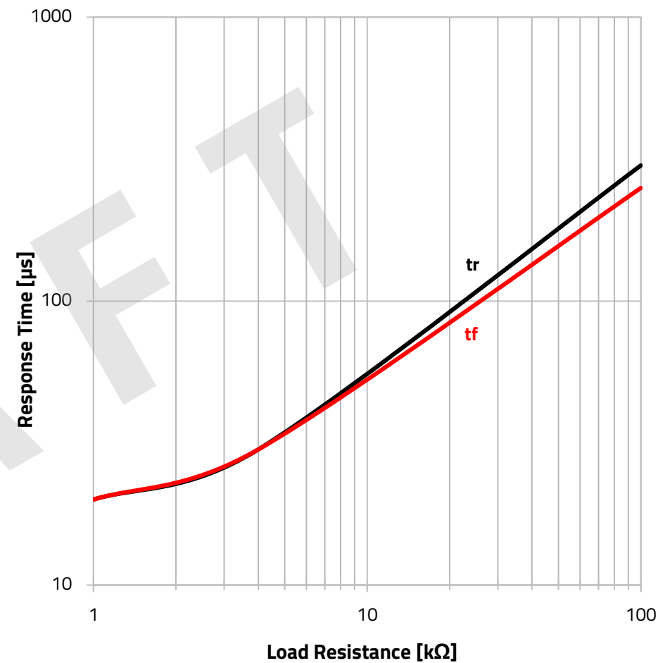
Switching time vs. Load Resistance:
