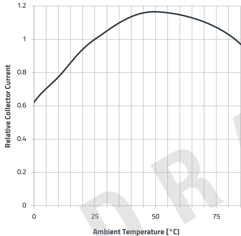
Collector Current vs. Ambient Temperature:
