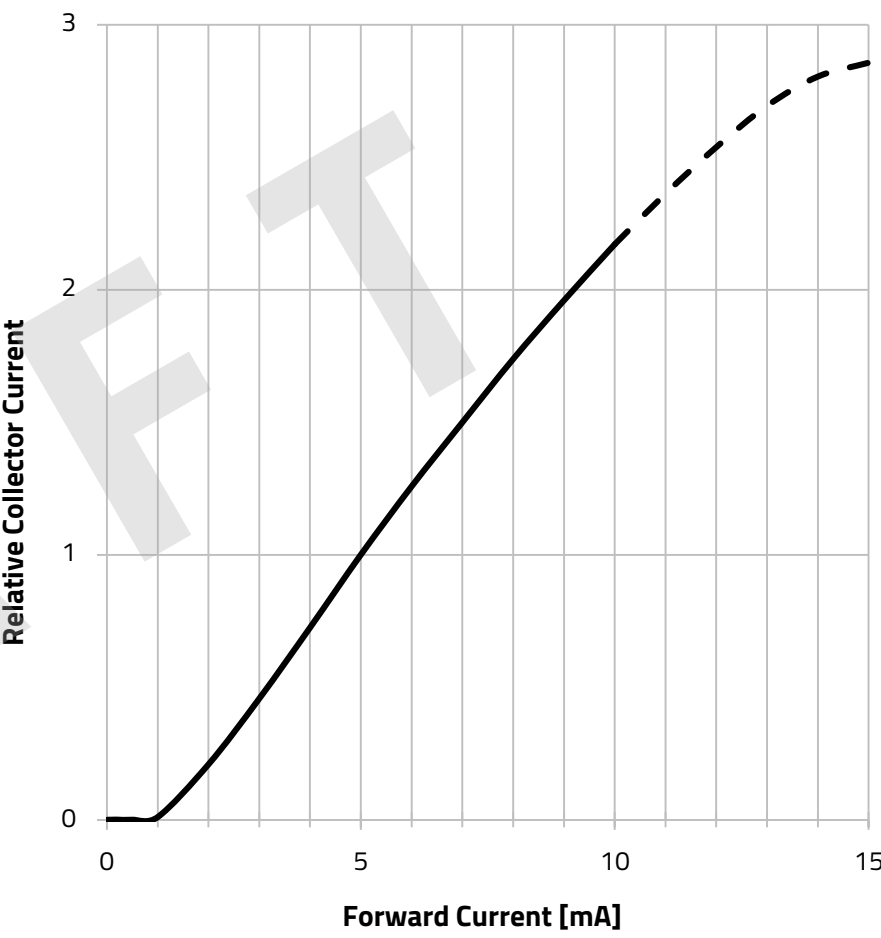
Relative Collector Current vs. Forward Current:
