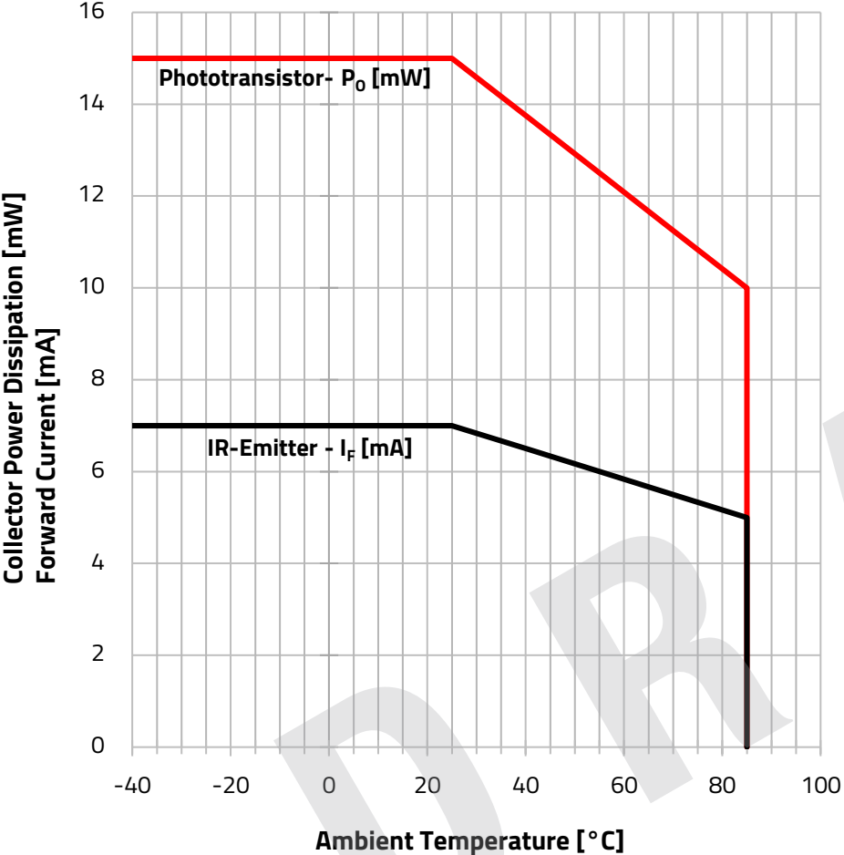
Derating Curve:
