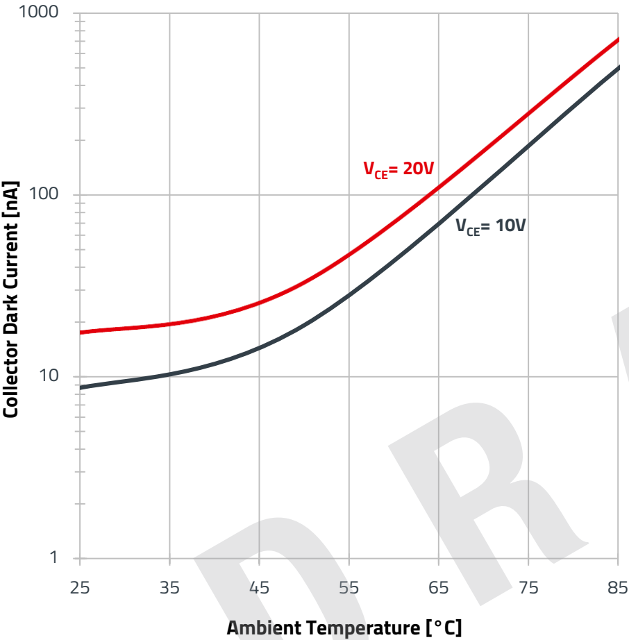
Collector Dark Current vs. Ambient Temperature:
