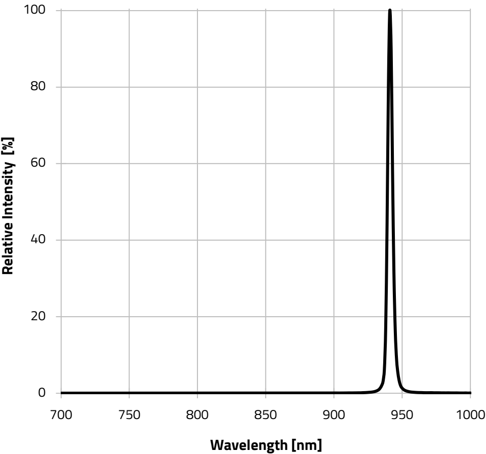
Spectral - Emitter
