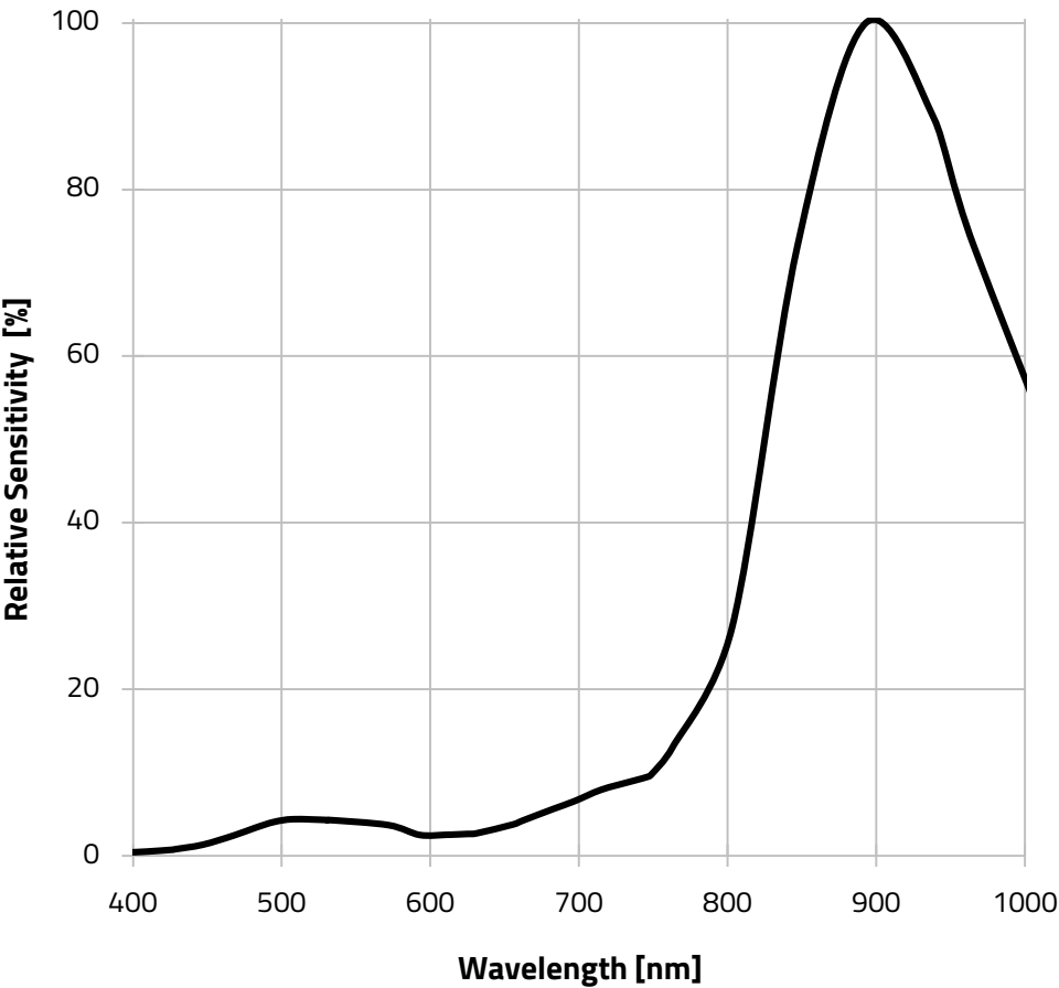
Spectral - Phototransistor
