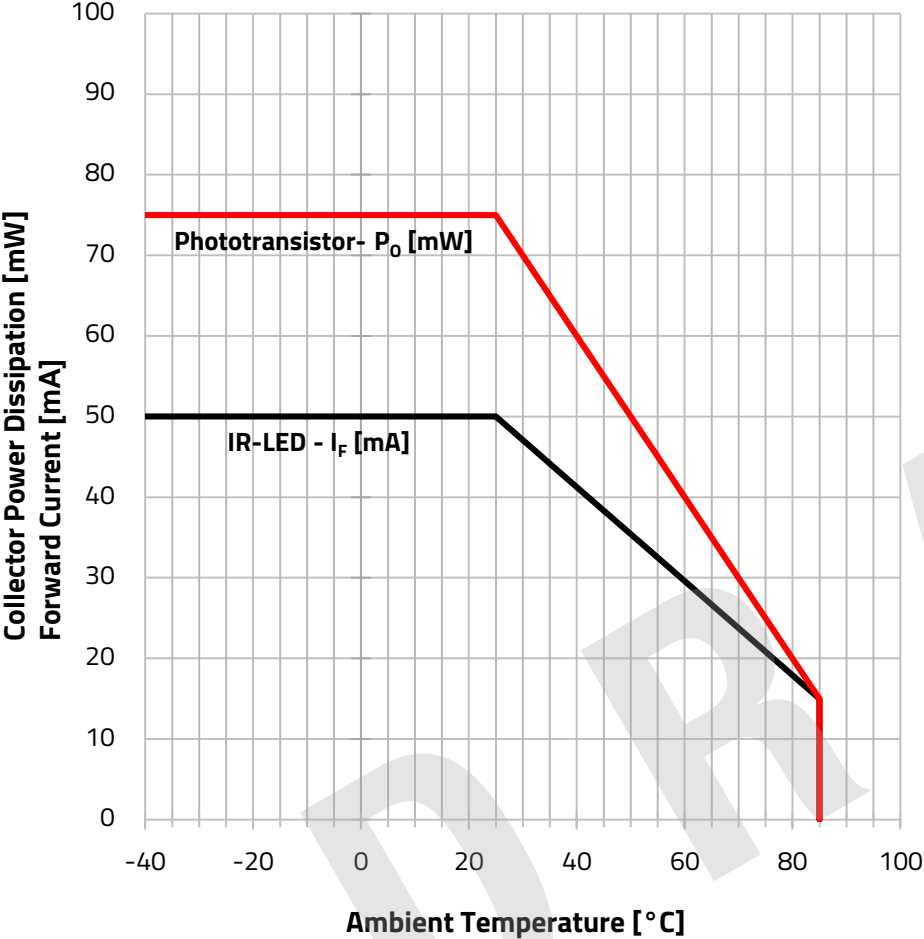
Derating Curve:
