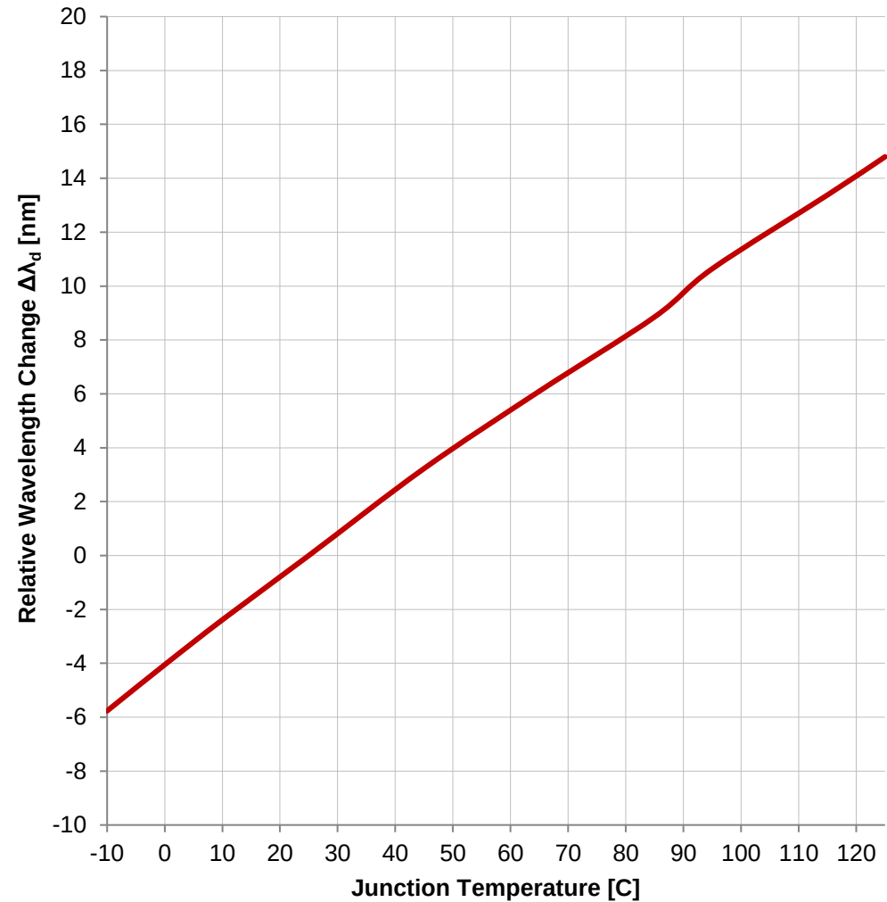
Junction Temperature vs. Dominant Wavelength:
