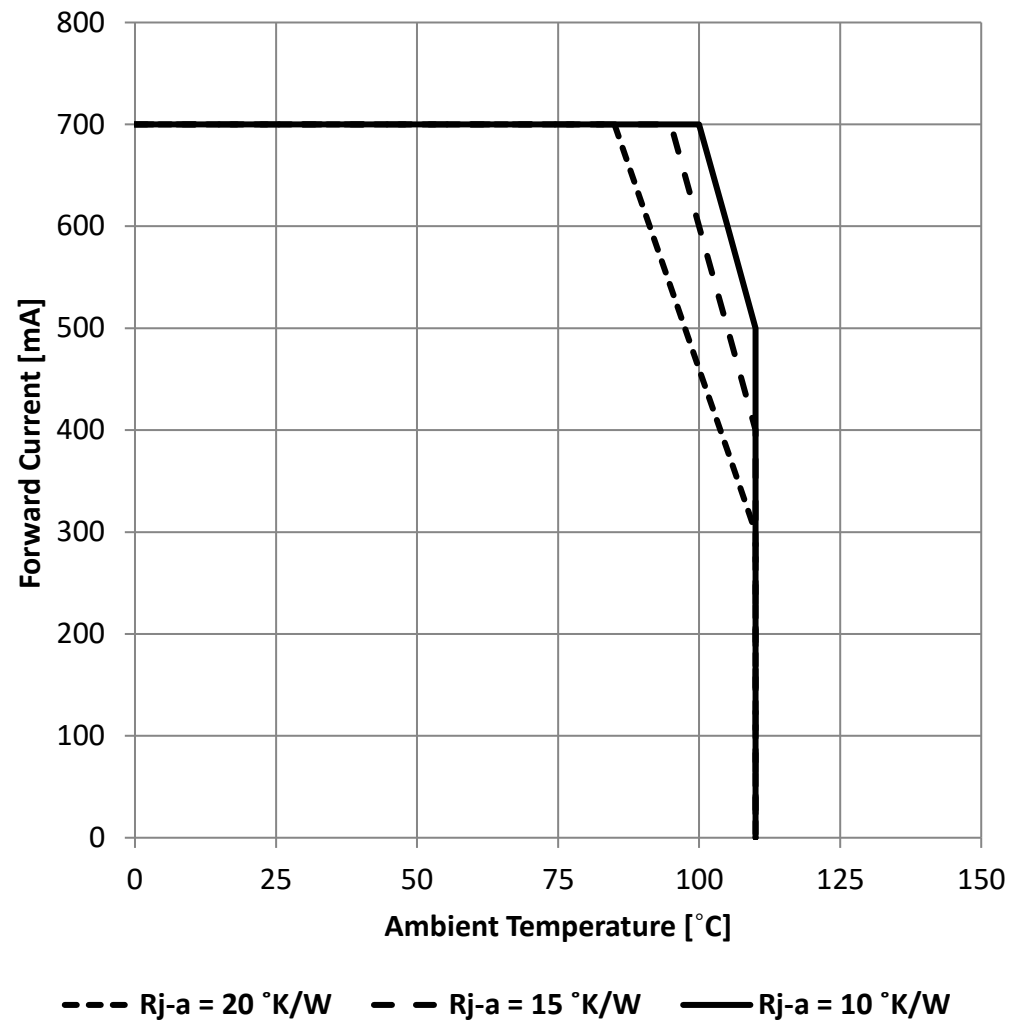
Derating Curve:
