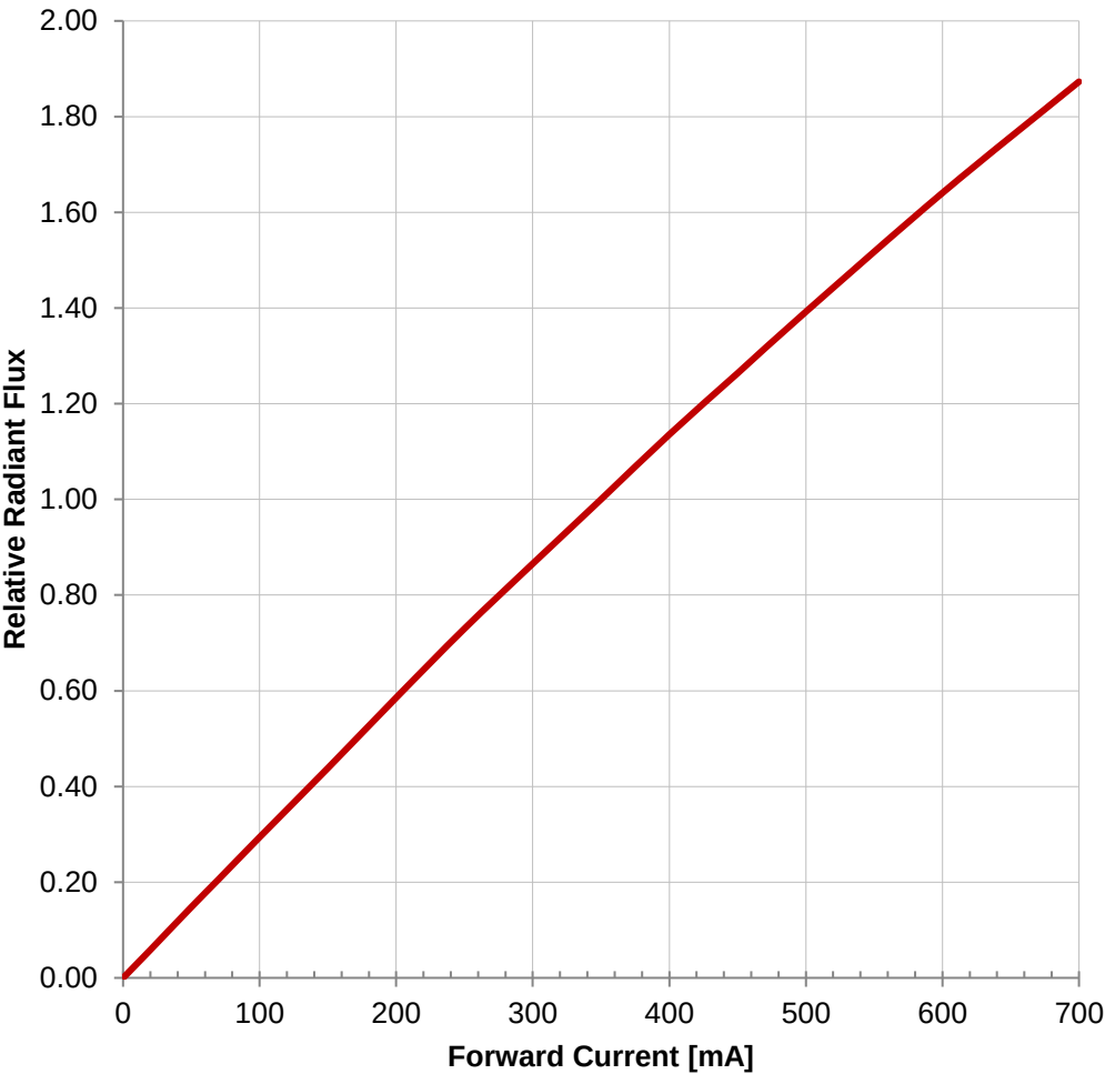
Radiant Flux vs. Forward Current:
