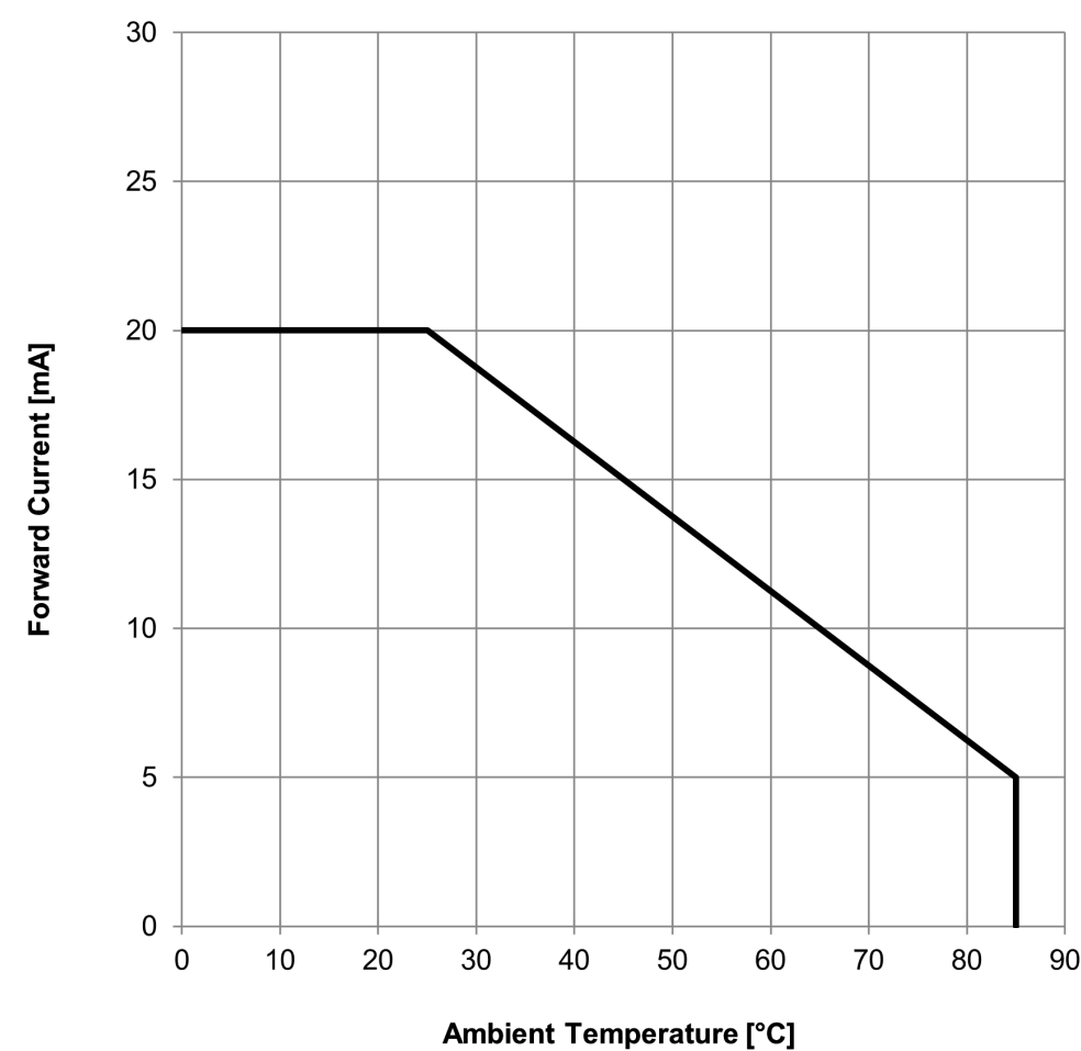
Derating Curve:
