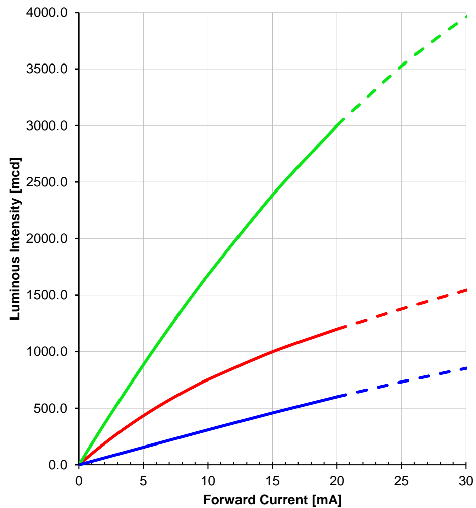
Luminous Intensity vs. Forward Current:
