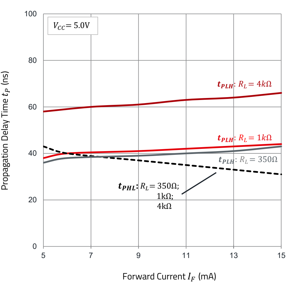
Propagation Delay Time vs. Forward Current:
