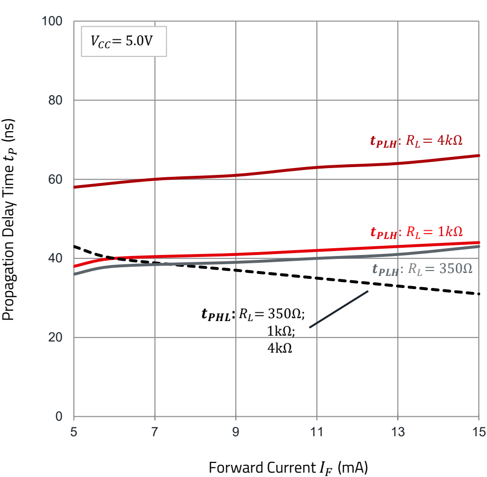
Propagation Delay Time vs. Forward Current:
