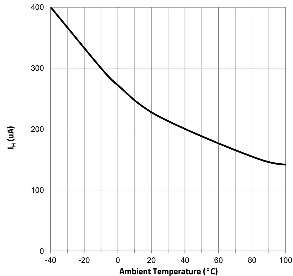
Holding Current vs. Ambient Temperature:
