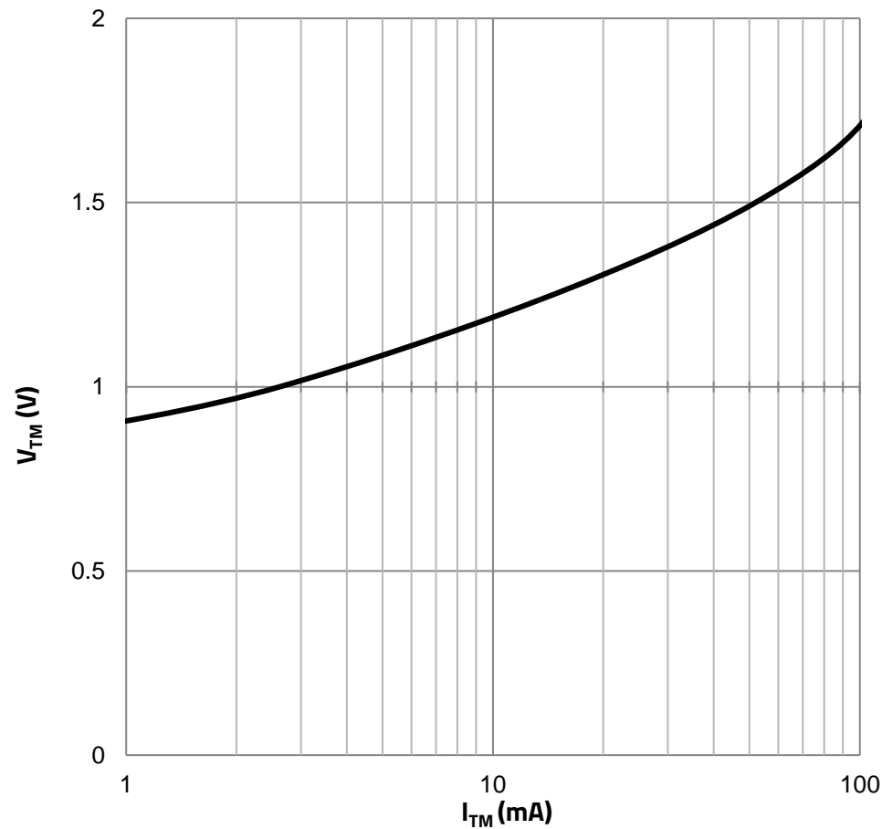
On-State Terminal Voltage vs. On-State Terminal Current:
