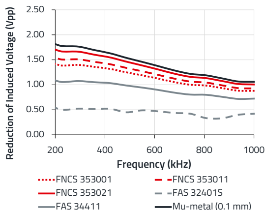
Figure 9: Calculated reduction of the induced voltage ( \text{Reduction} = V_{ref} - V_{shield} ) for different magnetic shielding materials vs frequency.
