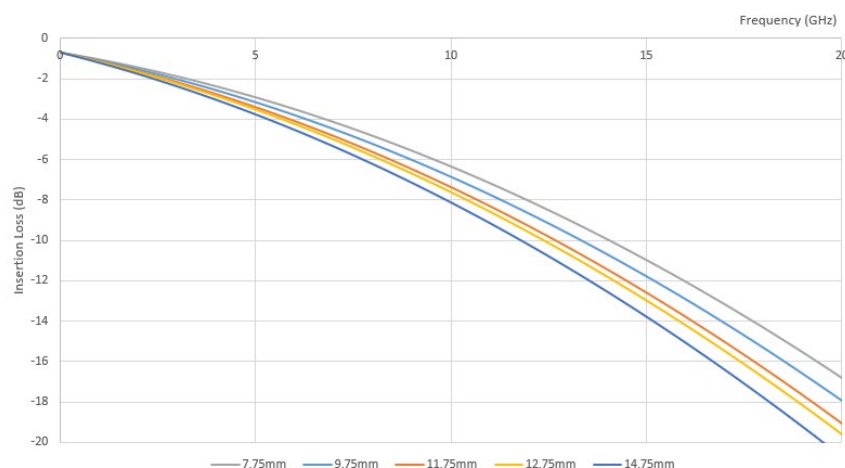
Figure 1: WR-BTB 1.0 mm Variable Mating Height Board-to-Board Connectors GSG 50 Ohm Insertion loss profile.
