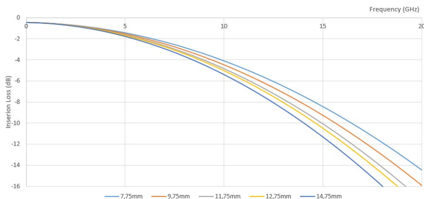
Figure 4: WR-BTB 1.0 mm pitch Variable Mating Height Board-to-Board Connectors GSSG 100 Ohm differential Insertion loss profile
