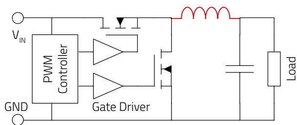
synchronous buck converter
