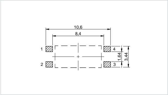
Recommended Land Pattern: [mm]
