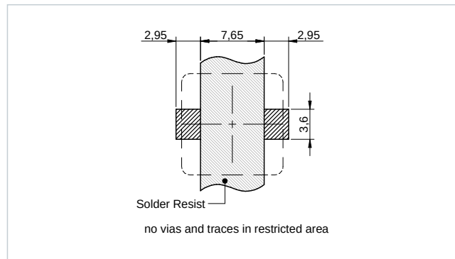
Recommended Land Pattern: [mm] 1212
