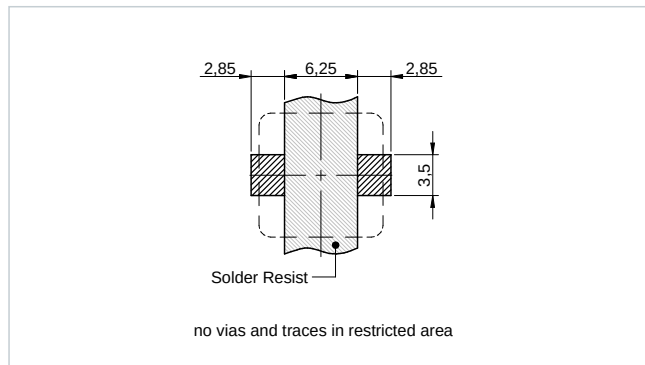
Recommended Land Pattern: [mm] 1011
