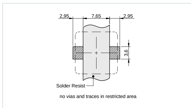
Recommended Land Pattern: [mm] 1212 P
