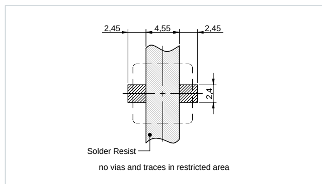
Recommended Land Pattern: [mm] 8090 P
