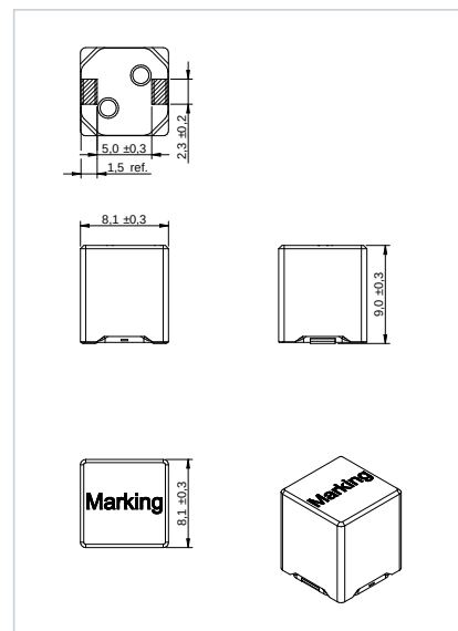
Dimensions: [mm] 8090 P
