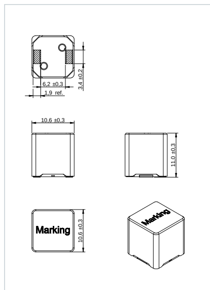
Dimensions: [mm] 1011 P
