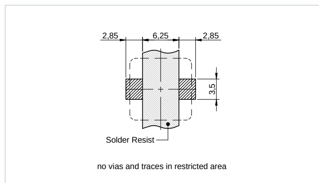
Recommended Land Pattern: [mm] 1011 P
