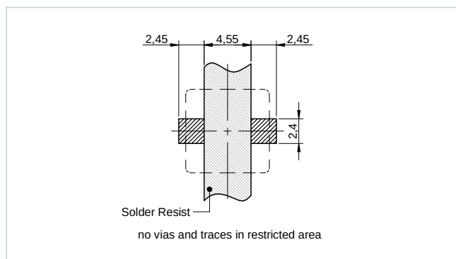
Recommended Land Pattern: [mm] 8090
