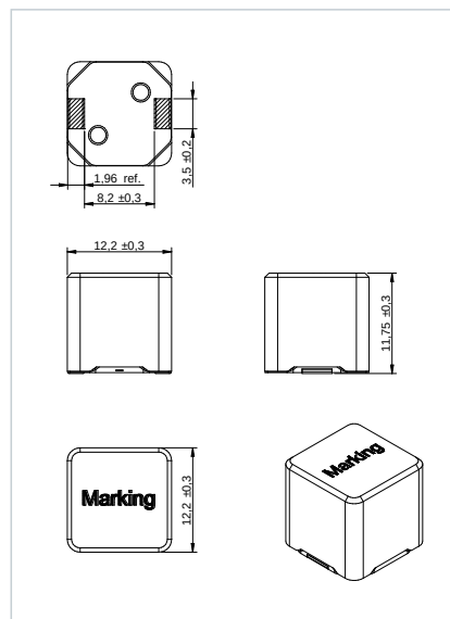
Dimensions: [mm] 1212 P
