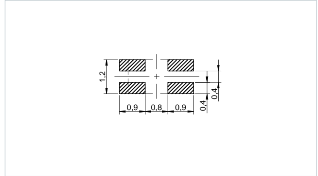
Recommended Land Pattern: [mm] Size 0805
