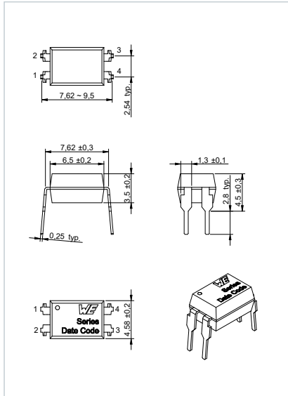
Dimensions: [mm] Standard
