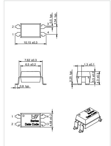
Dimensions: [mm] S
