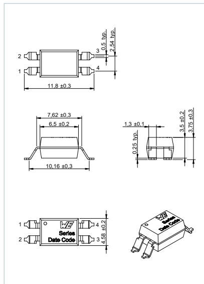
Dimensions: [mm] SLM
