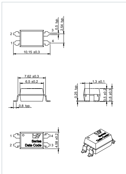
Dimensions: [mm] SL
