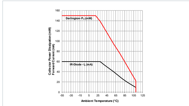
Derating Curve:
