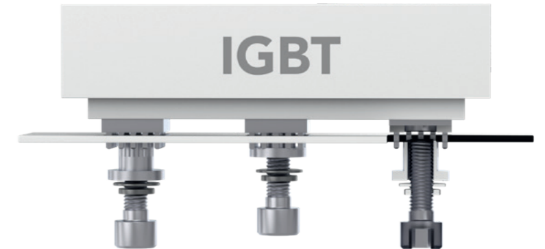
Two-part REDCUBE PRESS-FIT to mount IGBT
