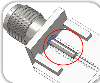
Figure 29: Original Design
