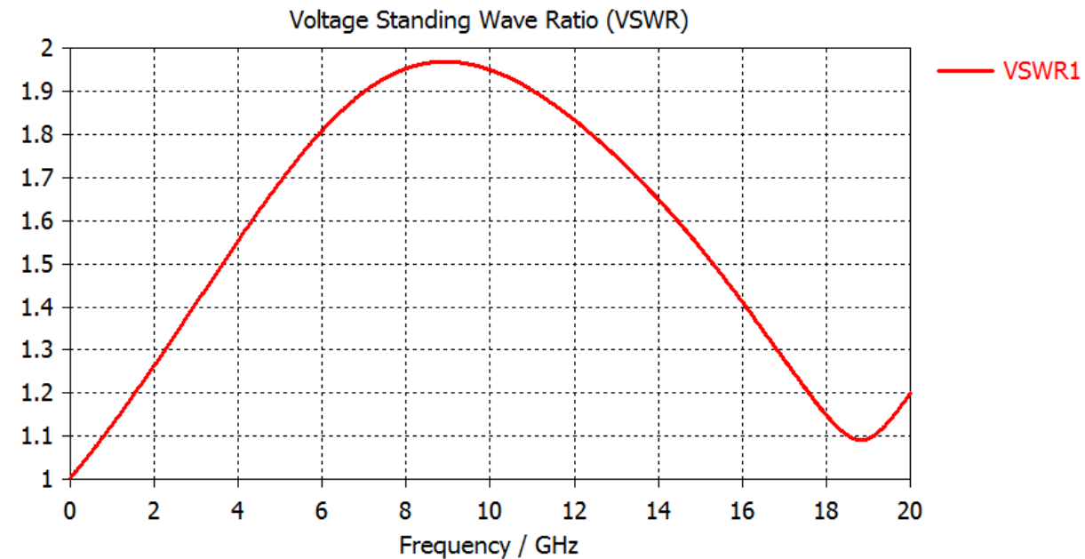
Figure 33: Result of S-Parameter – VSWR measurement (Original Design)
