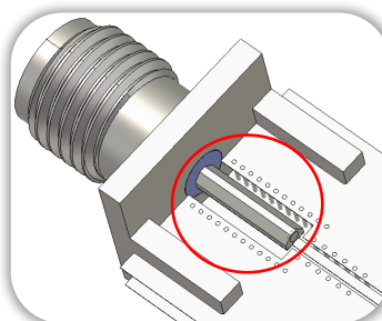
Figure 30: Matching Design
