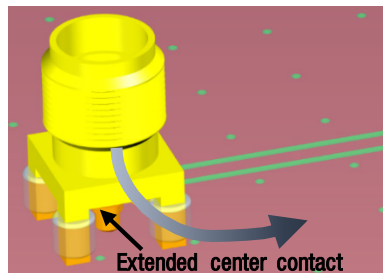
Figure 17: Signal route: Connector interface PCB trace
