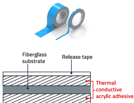
Figure 1: WE-TTT cross-section.
