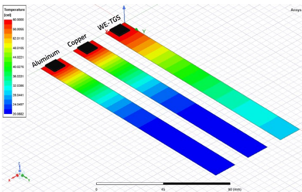
Figure 2: 18 x 18 mm strips with 5 W heat source.
