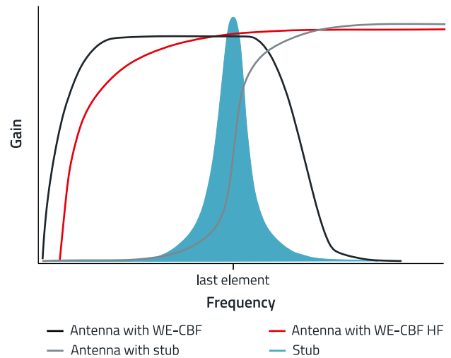
Figure 21: Gain over frequency of antenna with terminating stub.
