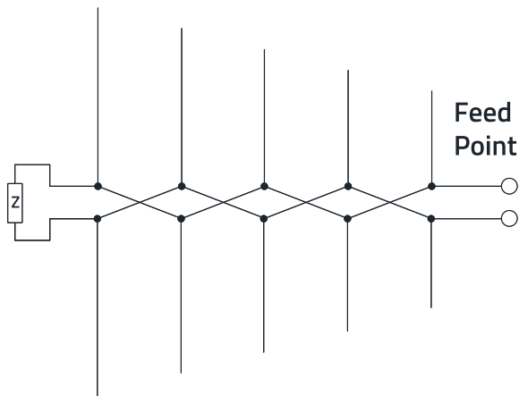
Figure 20: Diagram of a LPDA terminating with a high impedance.
