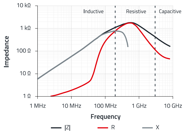
Figure 1: Impedance curve of WE-CBF HF (742841160).
