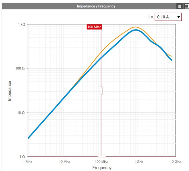
Figure 12: Interactive chart in REDEXPERT comparing WE-CBF HF 742861160 (blue) and 742863160 (orange) with 100 mA DC bias.
