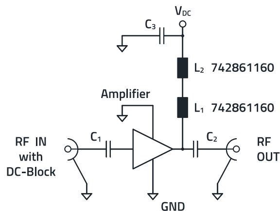
Figure 16: Gain amplifier circuit design.
