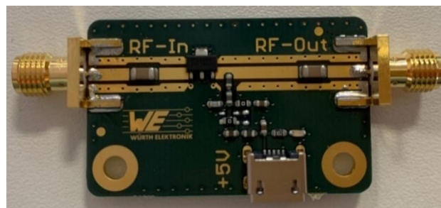
Figure 17: Gain amplifier test board with WE-CBF HF (742861160).
