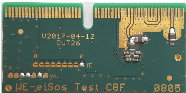
Figure 15: Test board of a SMT ferrite in case size 0805.
