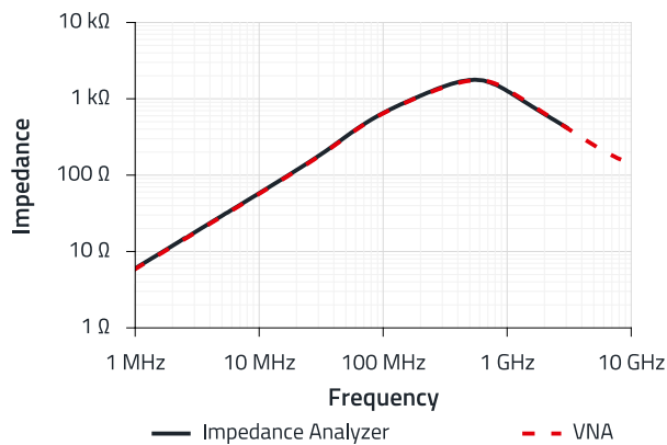
Figure 13: Graph showing a measurement of WE-CBF HF (742841160) from the impedance analyzer and VNA.
