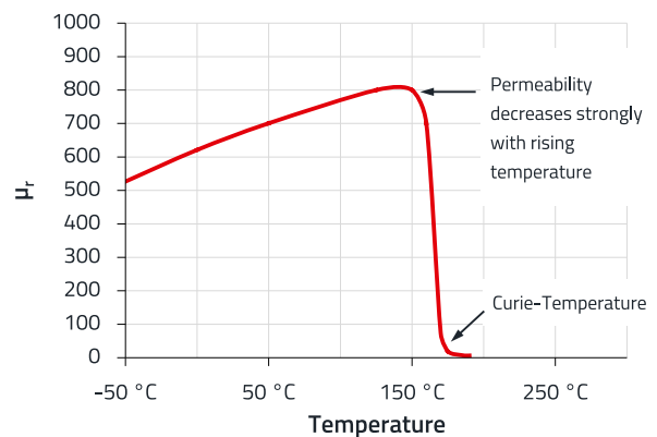
Figure 8: Curie temperature.
