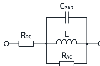
Figure 2: Equivalent circuit model.
