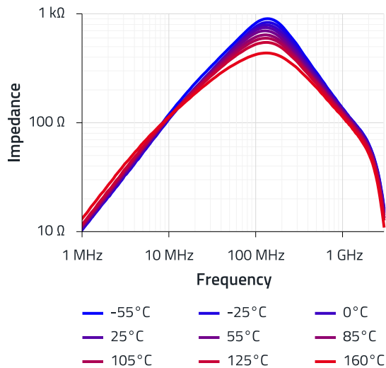
Figure 9: Impedance graph of WE-CBF 742792040 with temperature.
