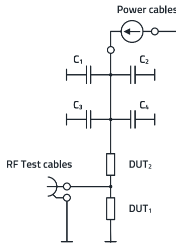
Figure 14: Würth Elektronik's enhanced test setup and circuit design.
