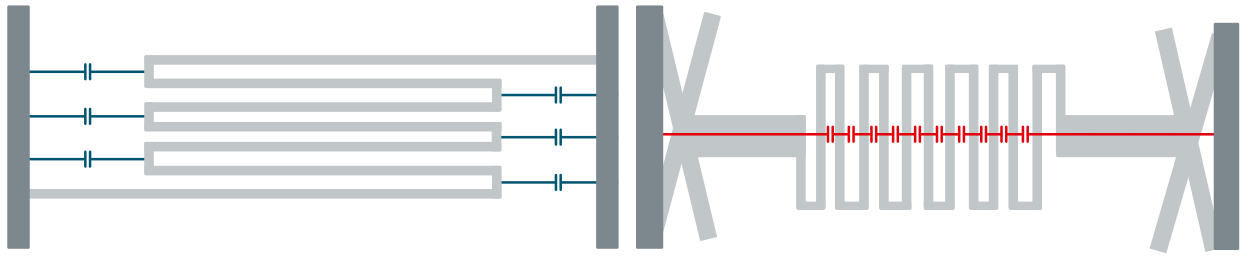
Figure 5: The parasitic capacitances of the WE-CBF (left) and WE-CBF HF (right).
