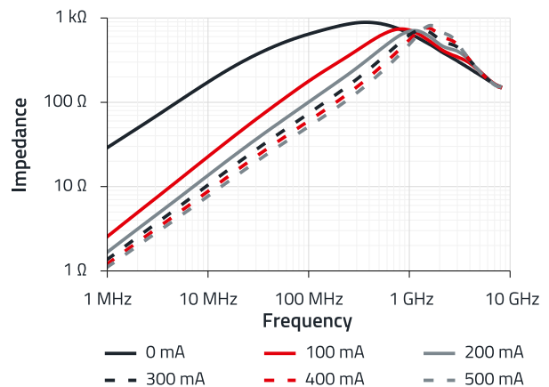
Figure 10: Comparison of the WE-CBF HF 742861160 under differing DC Bias conditions.
