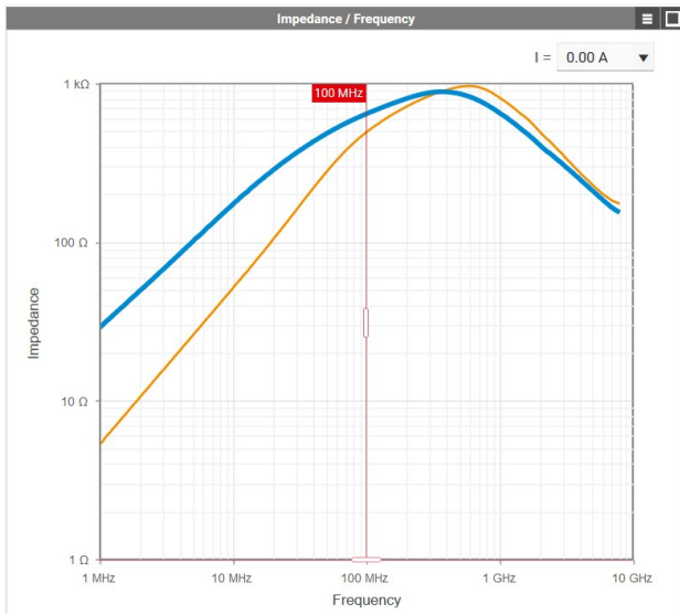
Figure 11: Interactive chart in REDEXPERT comparing WE-CBF HF 742861160 (blue) and 742863160 (orange) with 0 mA DC bias current.
