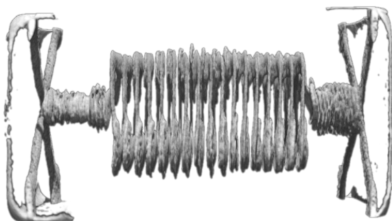
Figure 4: CT structure of vertical ferrite bead (WE-CBF HF).
