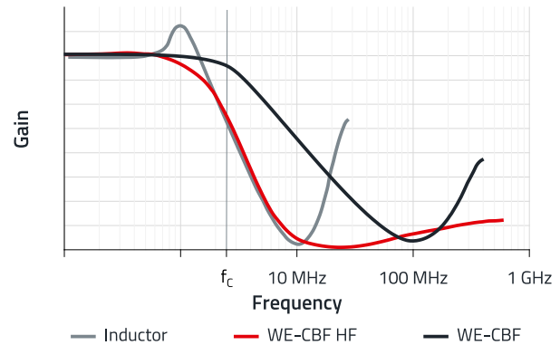
Figure 18: Gain response of a low pass filter for an inductor and ferrite beads.
