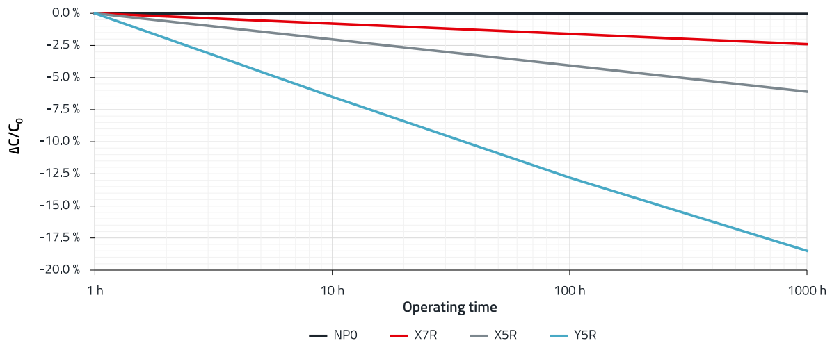
Figure 1: Capacitance loss vs. operating time
