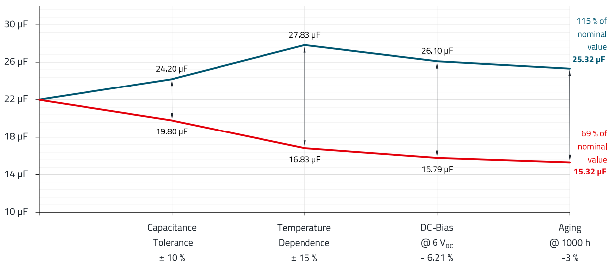
Figure 3: Real capacitance considering all dependencies
