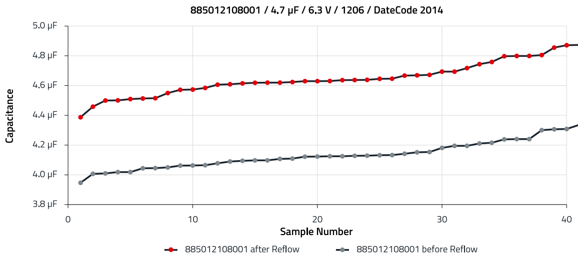
Figure 4: Capacitance measurement before (grey dots) and after (red dots) the reflow process
