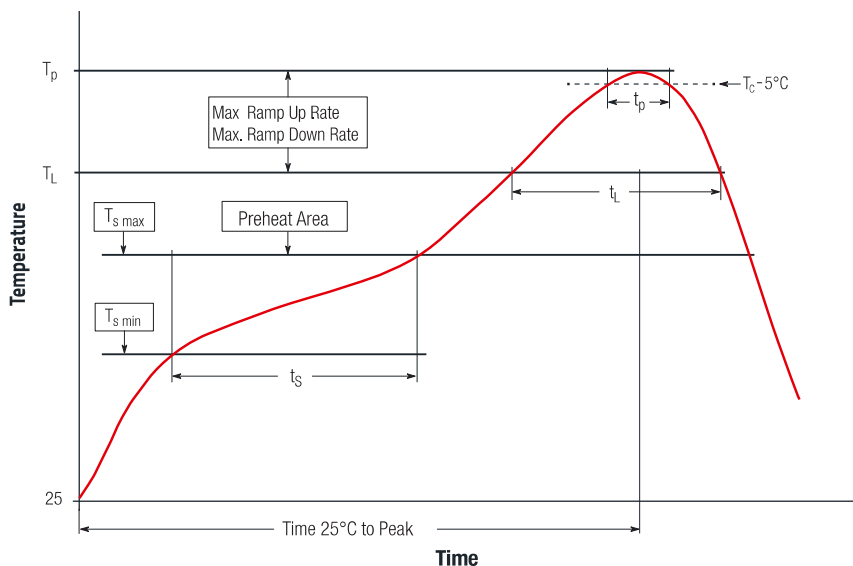
Figure 5: Soldering profile from the data sheet of the 885012108001
