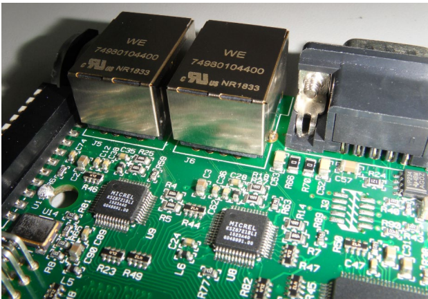
Abbildung 1: Demo Board.
