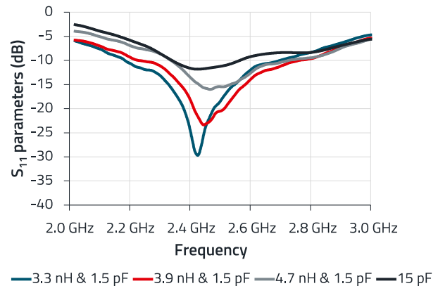
Figure 20: The effect of decreasing parallel inductance in the matching network of a WE-MCA Multilayer Chip Antenna.
