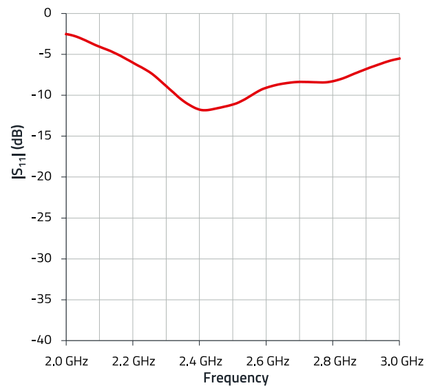
Figure 11: The S_{11} parameters of the shorted WE-MCA.
