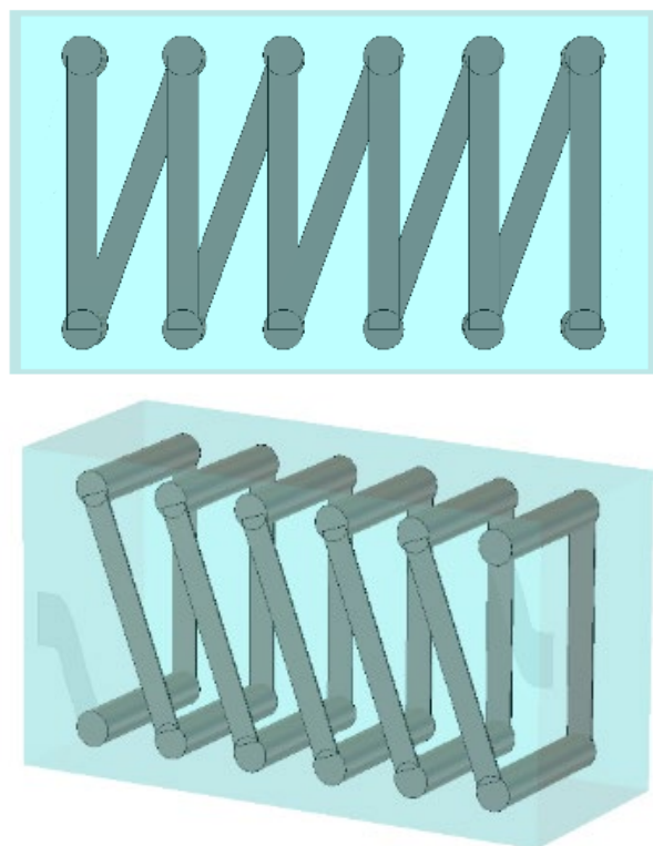
Figure 2: Internal structure of the WE-MCA Multilayer Chip Antenna ( 748 893 02 450 ).
