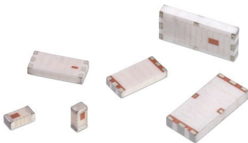
Figure 1: The WE-MCA Multilayer Chip Antenna.
