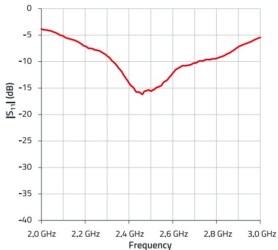
Figure 13: The S_{11} parameters of the partially matched WE-MCA .
