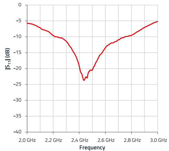
Figure 15: The S_{11} parameters of the sub-optimally matched WE-MCA .
