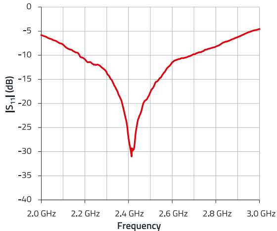
Figure 17: The S_{11} parameters of the optimally matched WE-MCA .
