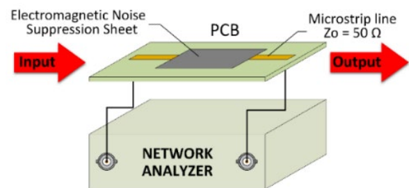
Figure 4: Microstrip Line Measurement System
