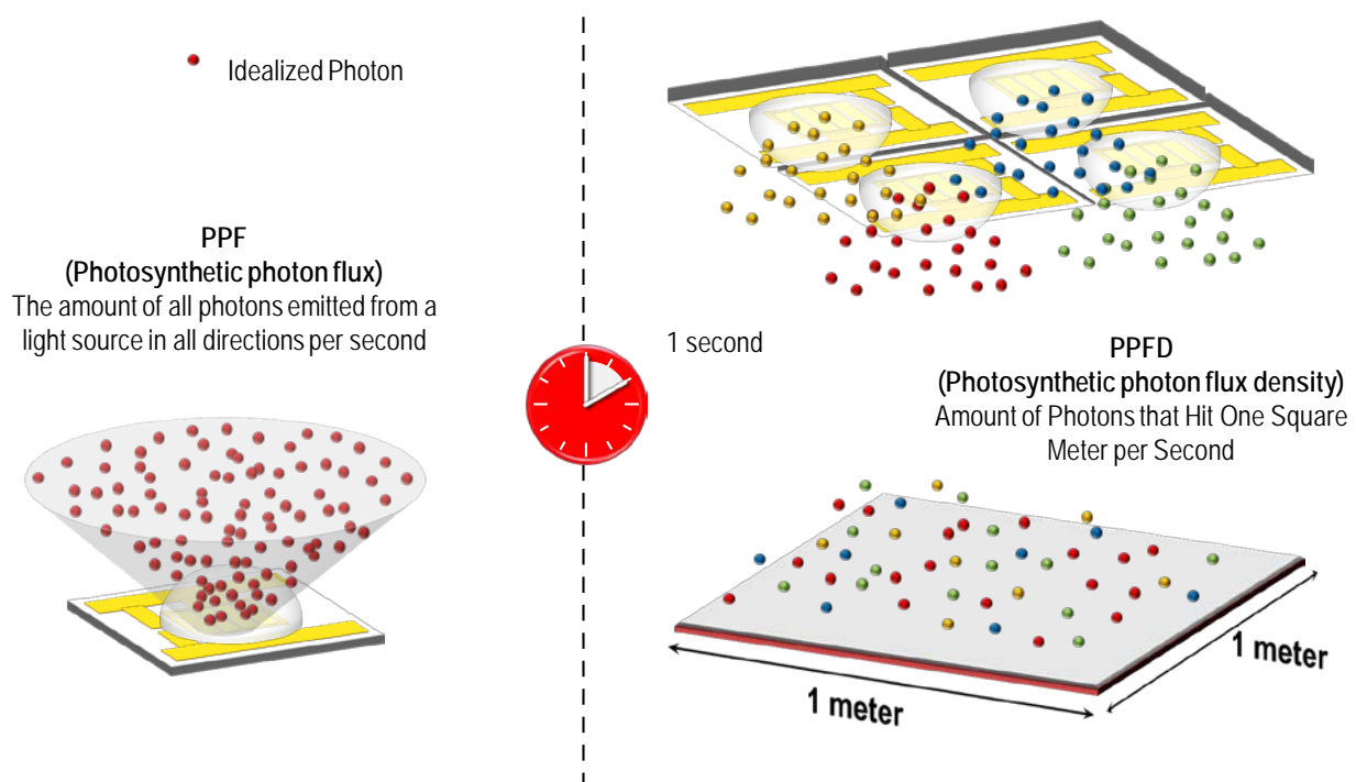
Figure 5: Photosynthetic Photon Flux (left) and Photosynthetic Photon Flux Density (right) with Several Colors
