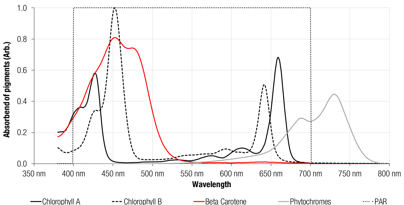
Figure 2: Characteristic Absorption Spectra of Different Pigments Used for Photosynthesis [1]
