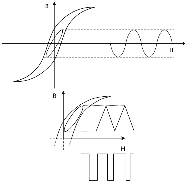
Figure 4: Typical modelling used for Steinmetz equation and its extensions on the top and Würth Elektronik's point of operation approach on the bottom
