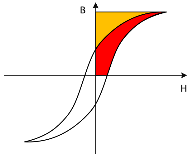
Figure 1: B-H Curve
