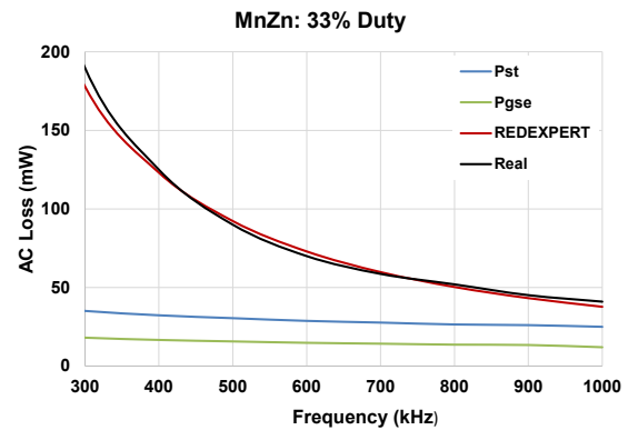
Figure 7: Inductor made of MnZn material at 33% DC
