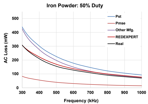
Figure 8: Inductor made of iron powder at 50% DC
