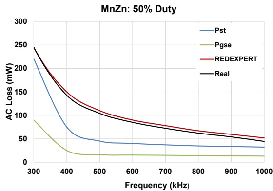
Figure 6: Inductor made of MnZn material at 50% DC
