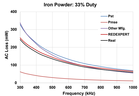
Figure 9: Inductor made of iron powder material at 33% DC
