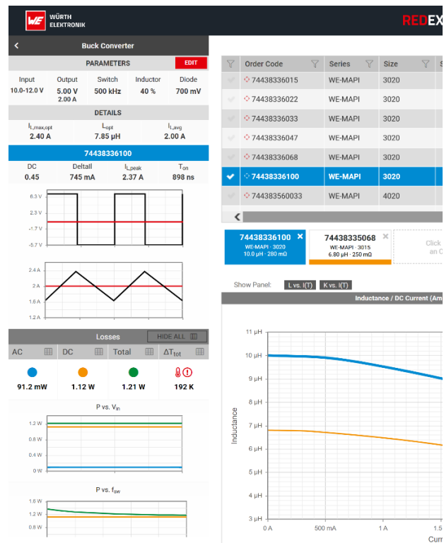
Figure 11: Buck-Converter Example
