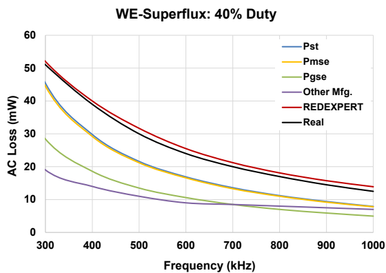
Figure 5: Inductor made of WE Superflux at 40% DC
