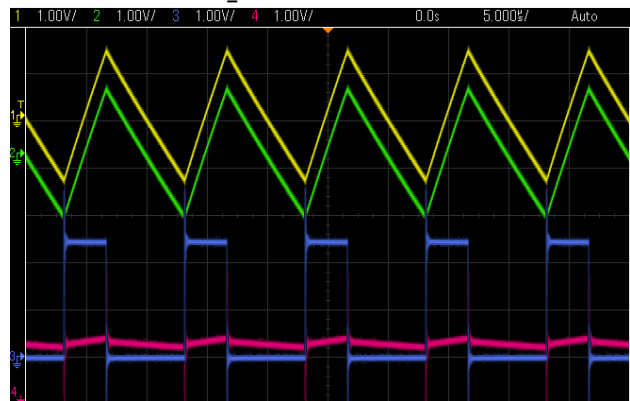
Figure 3: Setup of DC/DC converter for loss determination and resulting scope shots
