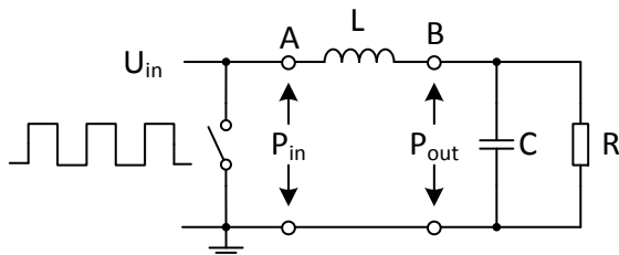
Fig 3: Setup of DC-DC Converter for Loss Determination and resulting scope shots
