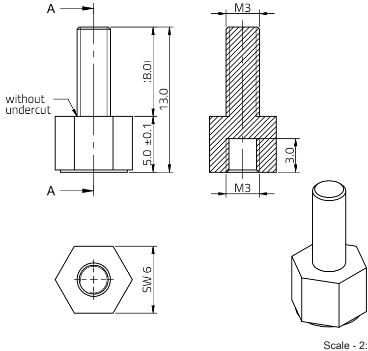
sectional drawing A-A
