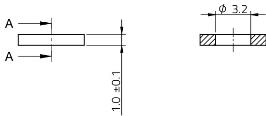
sectional drawing A-A
