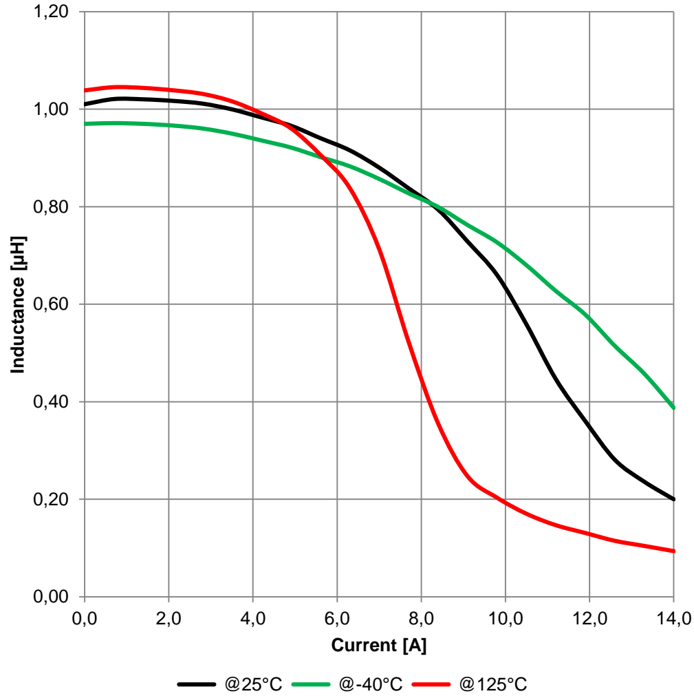
Typical Inductance vs. Current Characteristics - Three Turns:
