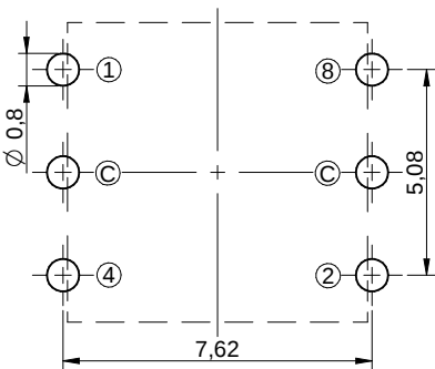
RECOMMENDED LAYOUT
