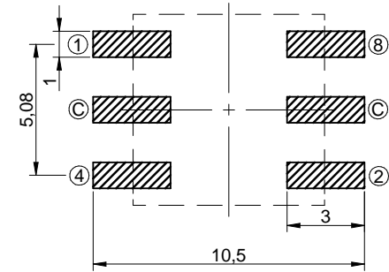
RECOMMENDED LAYOUT
