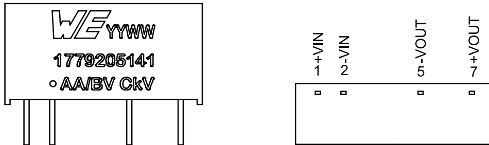
Figure 1: Pinout.
