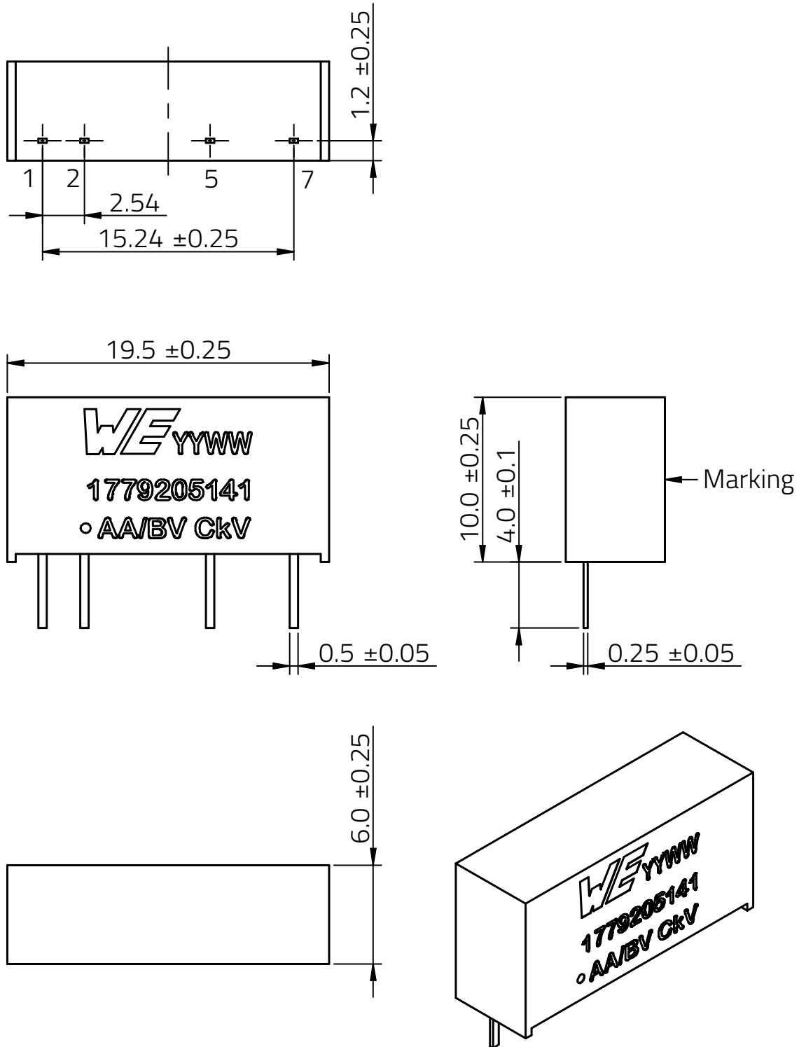
Figure 19: Component dimensions.
