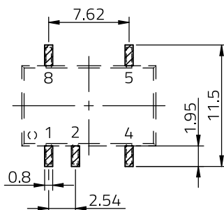
Figure 20: Recommended landpattern dimensions.
