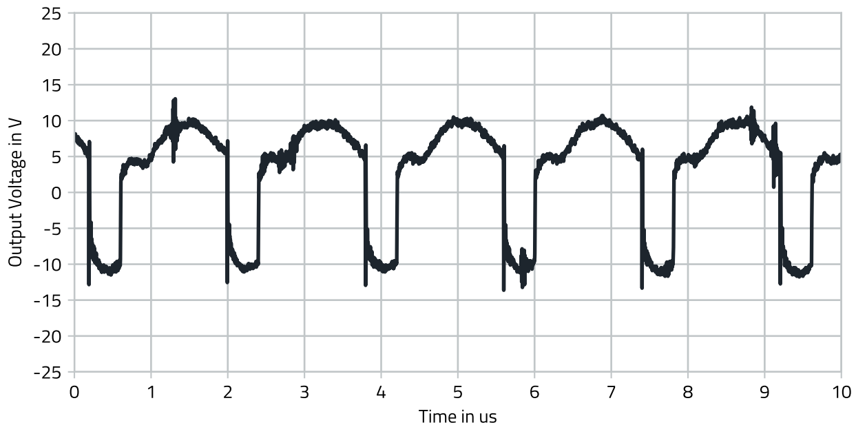
Figure 9: Output voltage ripple, V_{IN} = 24V , I_{OUT} = 1A .
