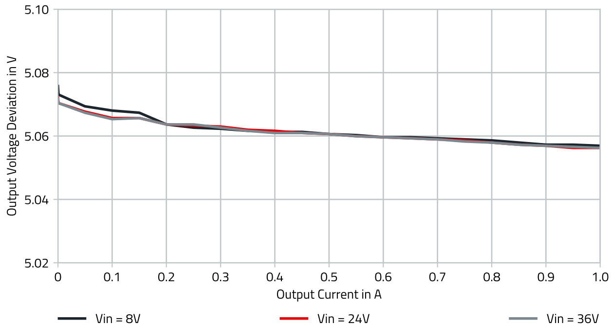
Figure 6: Load regulation.
