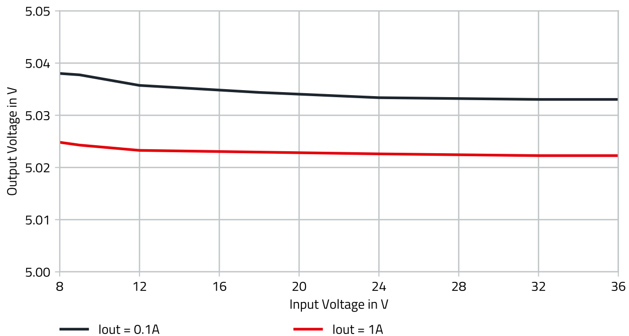
Figure 7: Line regulation.
