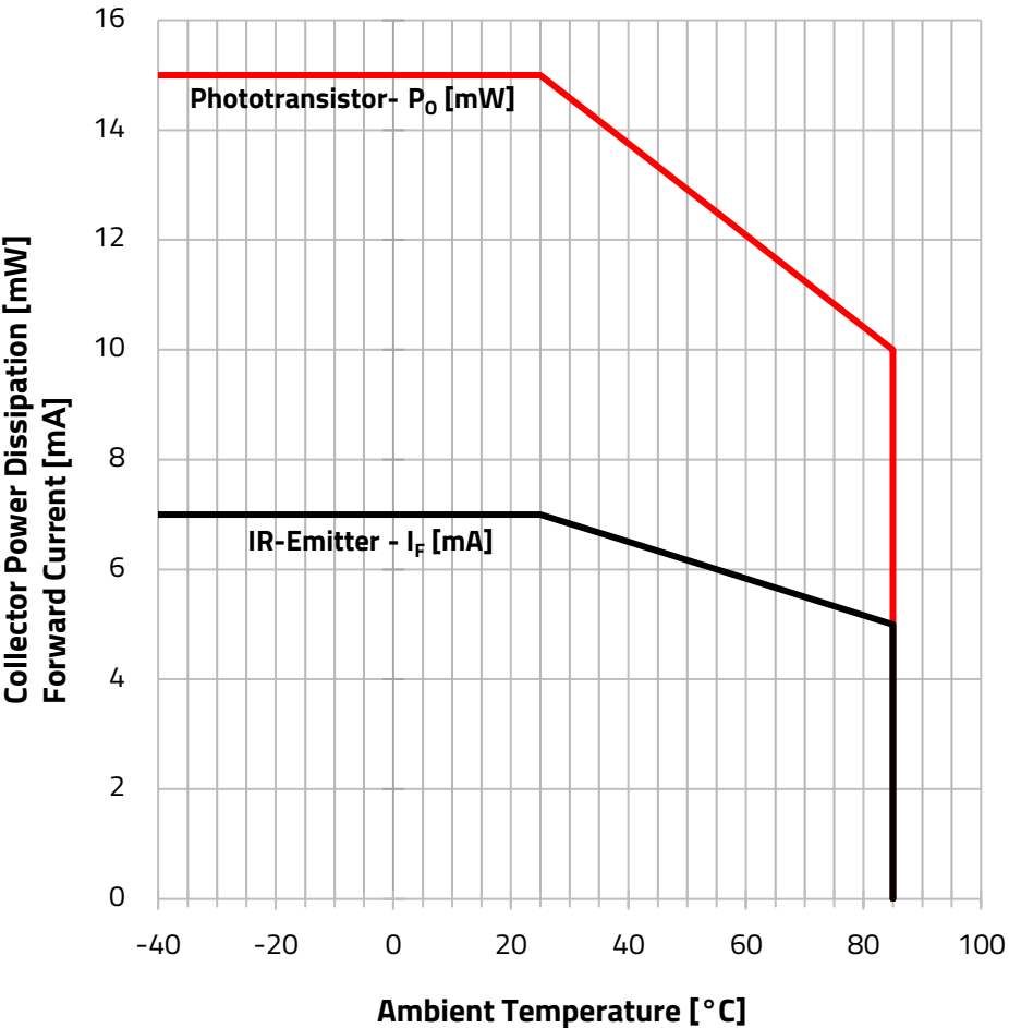
Derating Curve:
