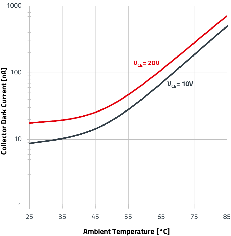
Collector Dark Current vs. Ambient Temperature:
