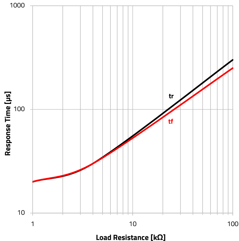
Switching time vs. Load Resistance:
