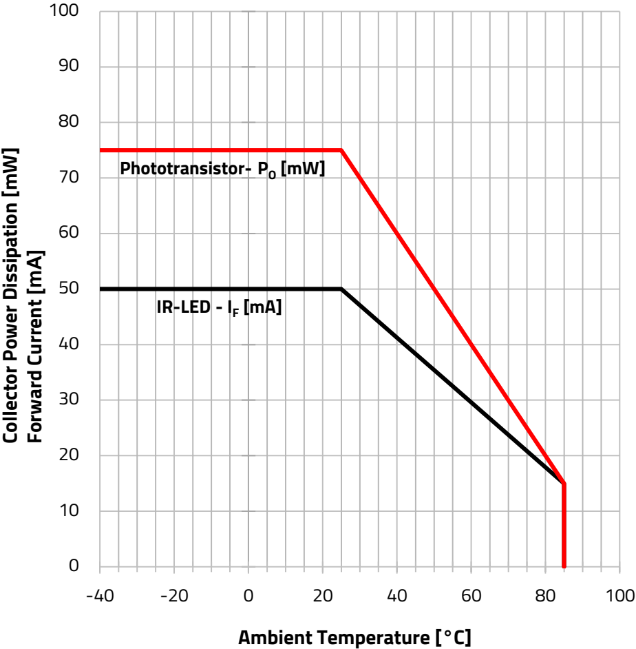
Derating Curve:
