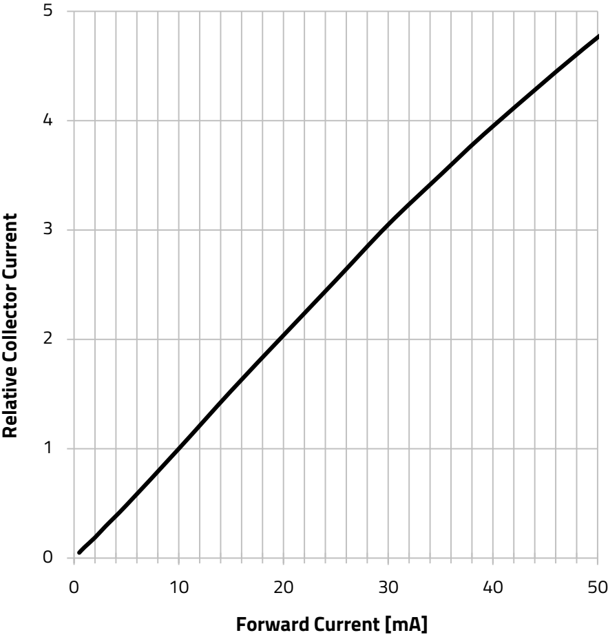
Relative Collector Current vs. Forward Current:
