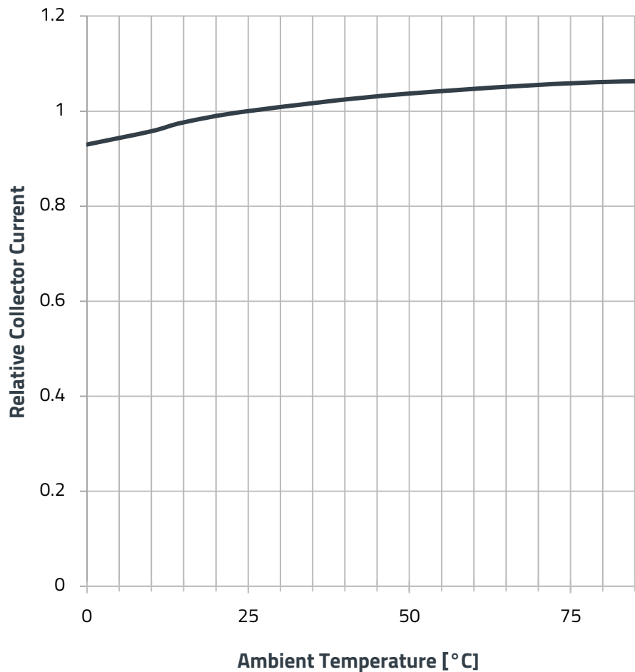
Collector Current vs. Ambient Temperature:
